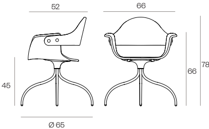
LOW BACKREST / SWIVEL BASE
