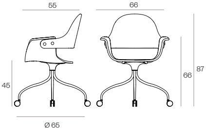
HIGH BACKREST / SWIVEL BASE WITH CASTERS
