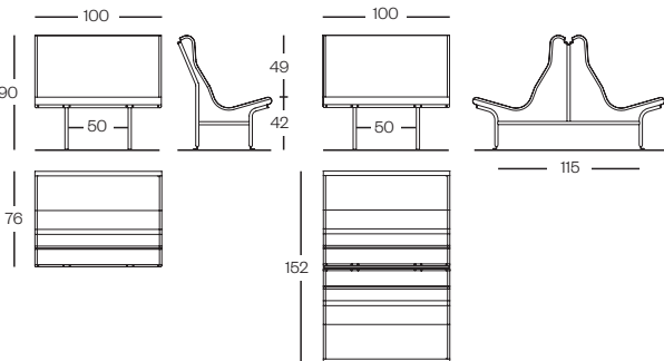
FREE-STANDING (TO BE SCREWED INTO THE FLOOR)
