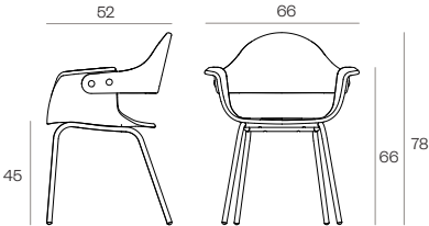
LOW BACKREST / METAL LEGS
