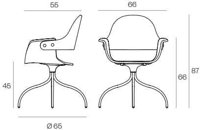
HIGH BACKREST / SWIVEL BASE
